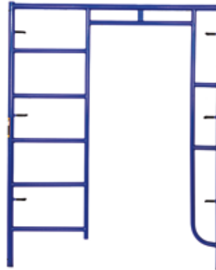
SWS-620B 5'X6'4" LADDER & WALK THRU FRAME WT. 52.40 LBS
