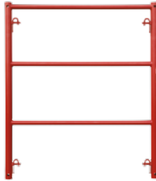
SWS-703 4'X5' SHORING FRAME WT. 52.60 LBS
