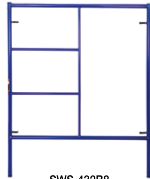
SWS-432B8 5'X6'4" DOUBLE LADDER WT. 42.60 LBS
