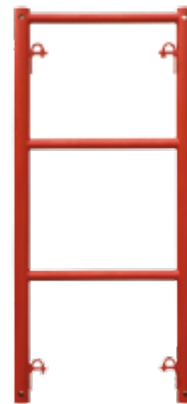
SWS-704 2'X5' SHORING FRAME WT. 45.40 LBS
