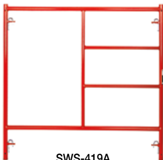
SWS-419A 5'X5'1" DOUBLE LADDER WT. 41.20 LBS
