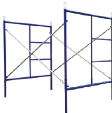
SWS-432B8-S 5'X6'4" S-STYLE DOUBLE LADDER FRAME SET (YELLOW) WT. 115.82 LBS
